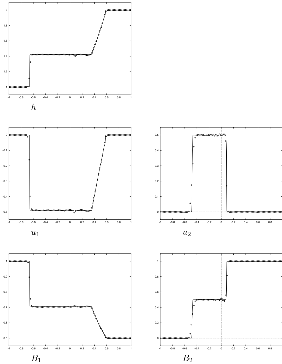
Figure 6.1: Numerical solution for the Riemann problem with 100 \times 5 cells (dots) and 1000 \times 5 cells (solid line).
