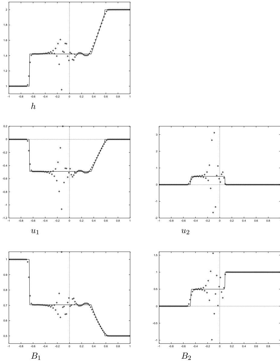
Figure 6.2: Numerical solution for the Riemann problem with 100 \times 5 cells using variant 2 of Subsection 6.1.
