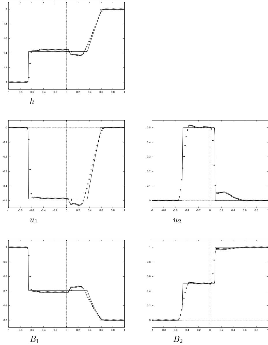
Figure 6.3: Numerical solution for the Riemann problem with 100 \times 5 cells using variant 3 of Subsection 6.1.
