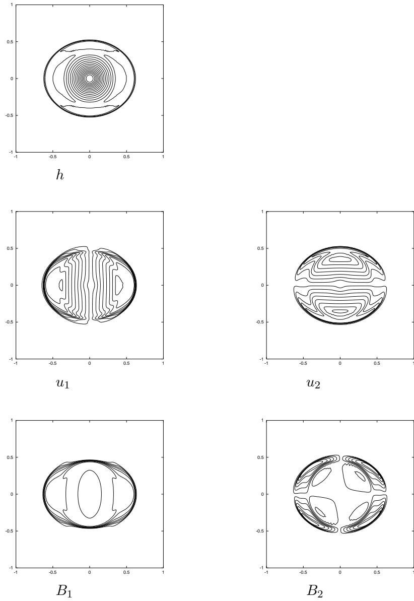
Figure 6.6: Contour plots of the two-dimensional explosion problem with 200 \times 200 cells.
