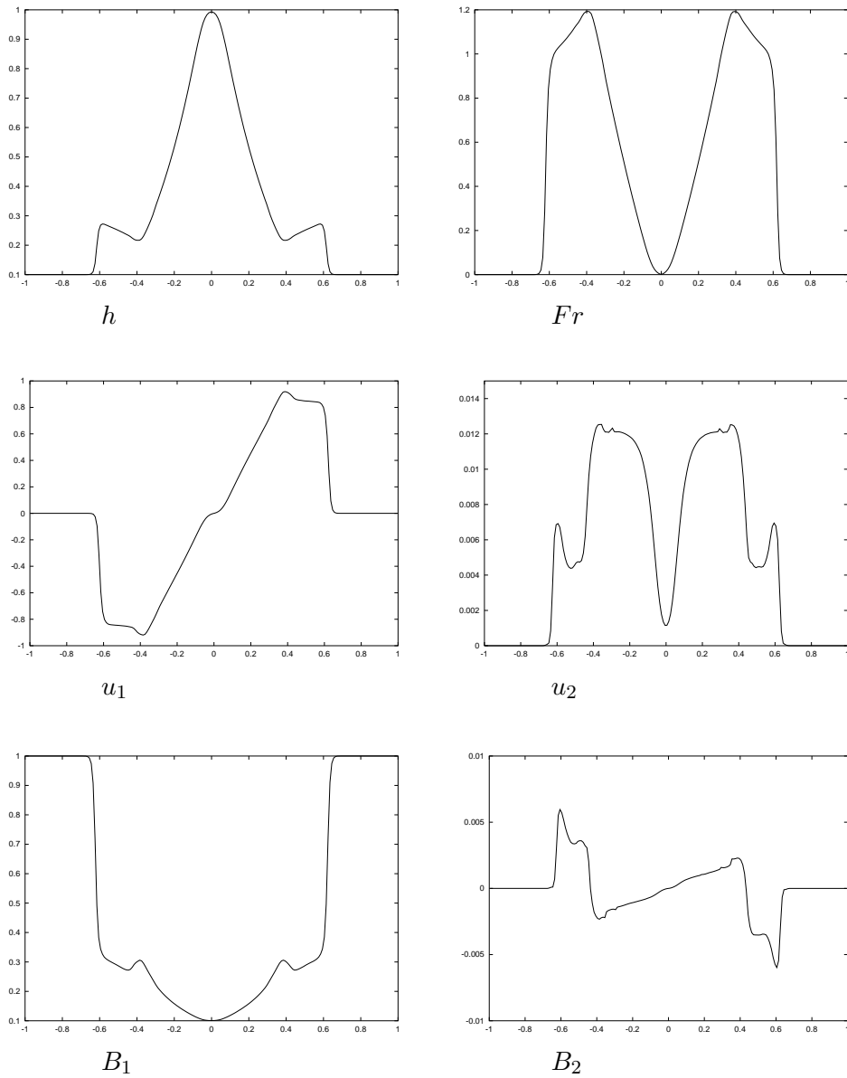
Figure 6.7: Graph of the solution of the two-dimensional explosion problem with 200 \times 200 cells, cross section for y = 0 .
