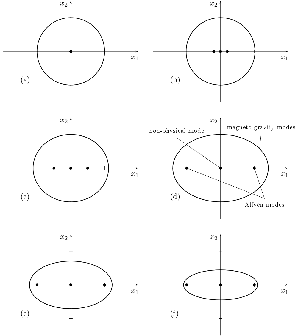
Figure 3.1: Friedrichs diagrams for SMHD equations for \underline{u} = \underline{0} , g = 1 , and (a) h = 1, \underline{B} = (0, 0) , (b) h = 1, \underline{B} = (0.2, 0) , (c) h = 1, \underline{B} = (0.5, 0) , (d) h = 1, \underline{B} = (1, 0) , (e) h = 0.5, \underline{B} = (1, 0) , (f) h = 0.2, \underline{B} = (1, 0) .
