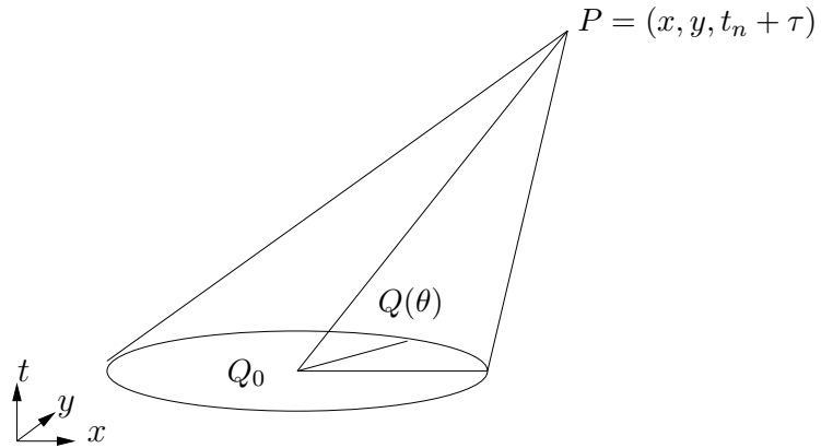
Figure 1: Bicharacteristics cone.
