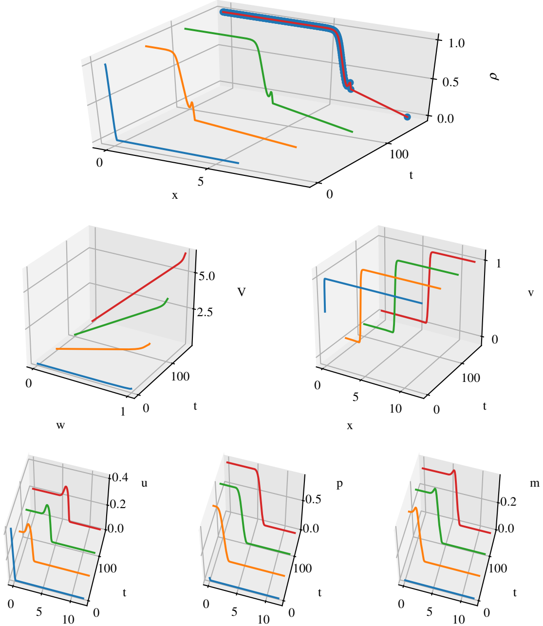
FIGURE 10. Numerical results (cancer cell concentration, inverse cumulative function, ECM, uPA, PAI-1 and plasmin density in space and time) in the model (4.14) with volume filling by (4.15) and exponent \gamma = 0.5 . We have used M = N = 400 grid points on both meshes in the numerical simulation.
