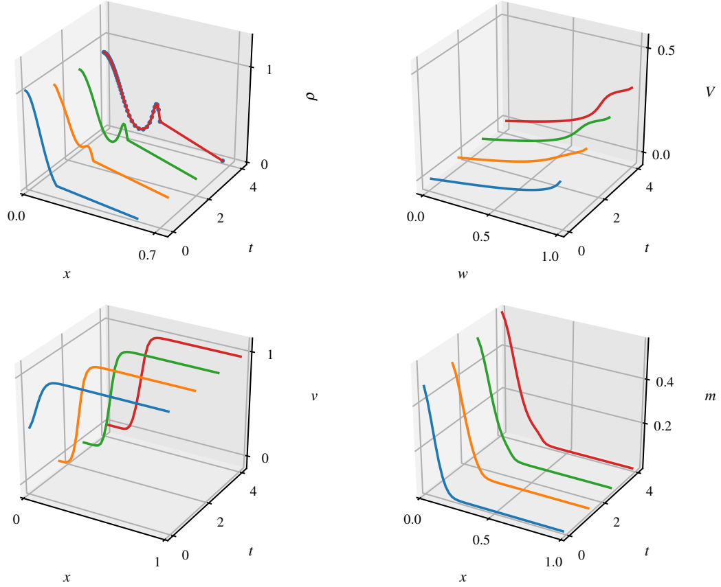
FIGURE 7. Numerical results (cell concentration, inverse cumulative function, tissue and MMP density) for the cancer invasion model (4.11) using only N = M = 45 mesh points. At the final time we show the approximated cell averages of the tumor density \rho at their respective position on the grid (top left). A high concentration of tumor cells emerges and invades the tissue. The grid for the tumor density omits the part of the tissue that is not yet invaded.
