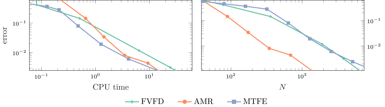
FIGURE 11. Relation between the CPU time and the error (left) and between the (average) number of cells and the error (right) for the FVFD, AMR, and MTFE scheme in log-log scale in a numerical experiment with the uPA model (4.14). The new MTFE method seems to be most efficient in terms of error per CPU time, its relation between the error and the average number of cells is similar as in the FVFD scheme.
