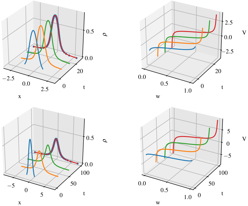
FIGURE 4. Numerical results (cell concentration, inverse cumulative function) for the model (4.6) with chemo-attractant given by a convolution as in (4.1). Results are shown for \gamma = 2 (top row) and \gamma = 0.5 (bottom row). We have used M = 50 points in the numerical computation.
