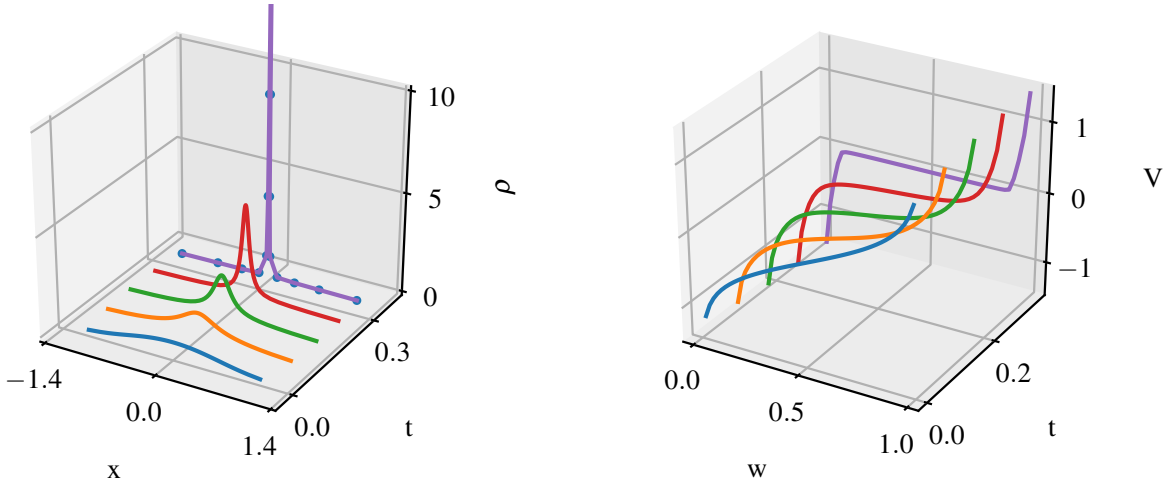
FIGURE 1. Numerical results (cell concentration and inverse cumulative function) for the parabolic elliptic Keller-Segel model, experiment 4.3.1 in [3]. The cell concentration blows up. The numerical cell concentration has attained a maximum of approximately 176.
