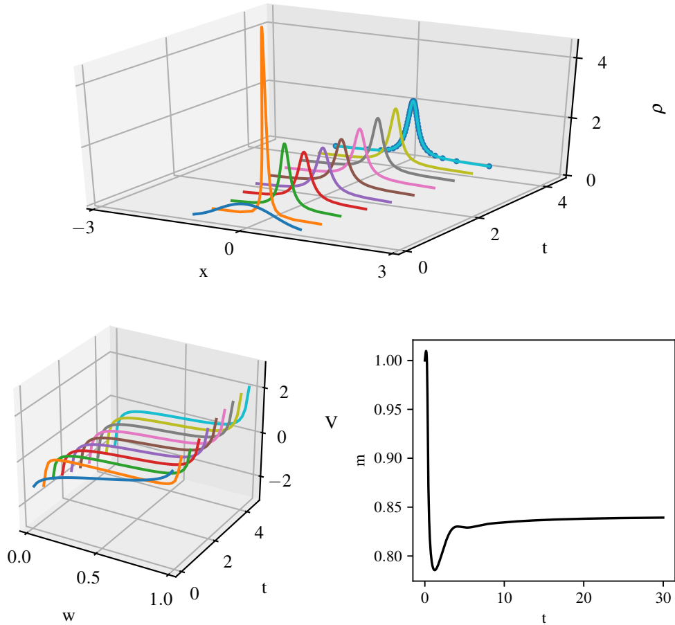
FIGURE 2. Numerical results (cell concentration, inverse cumulative function, and mass) for the parabolic elliptic Keller-Segel model with added logistic growth (4.1). The additional reaction term has prevented blowup.
