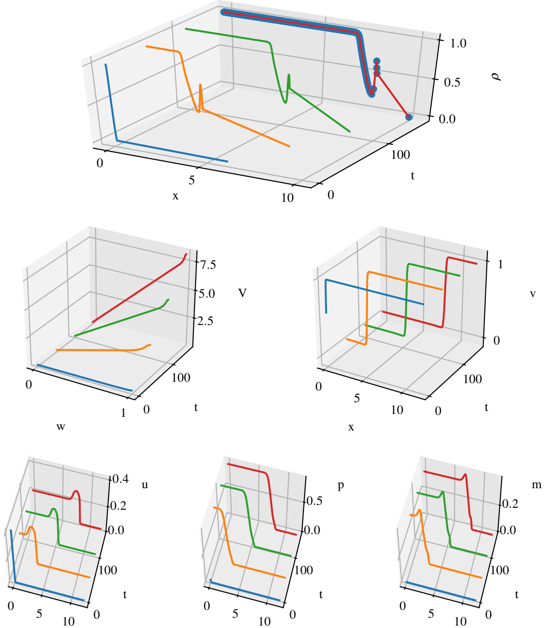
FIGURE 9. Numerical results (cancer cell concentration, inverse cumulative function, ECM, uPA, PAI-1 and plasmin density in space and time) in the model (4.14) with volume filling by (4.15) and exponent \gamma = 2 . We have used M = N = 400 grid points on both meshes in the numerical simulation.
