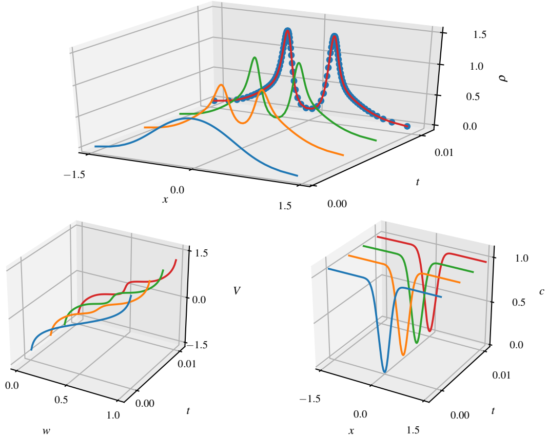
FIGURE 6. Numerical results (cell concentration, inverse cumulative function, and chemo-attractant density in space and time) for the parabolic-parabolic KS model (4.8) in the “peak splitting” experiment. At the final time we show the approximated cell averages of the density \rho at their respective position on the grid (top). The grid for the cell density adapts to the two splitting peaks.
