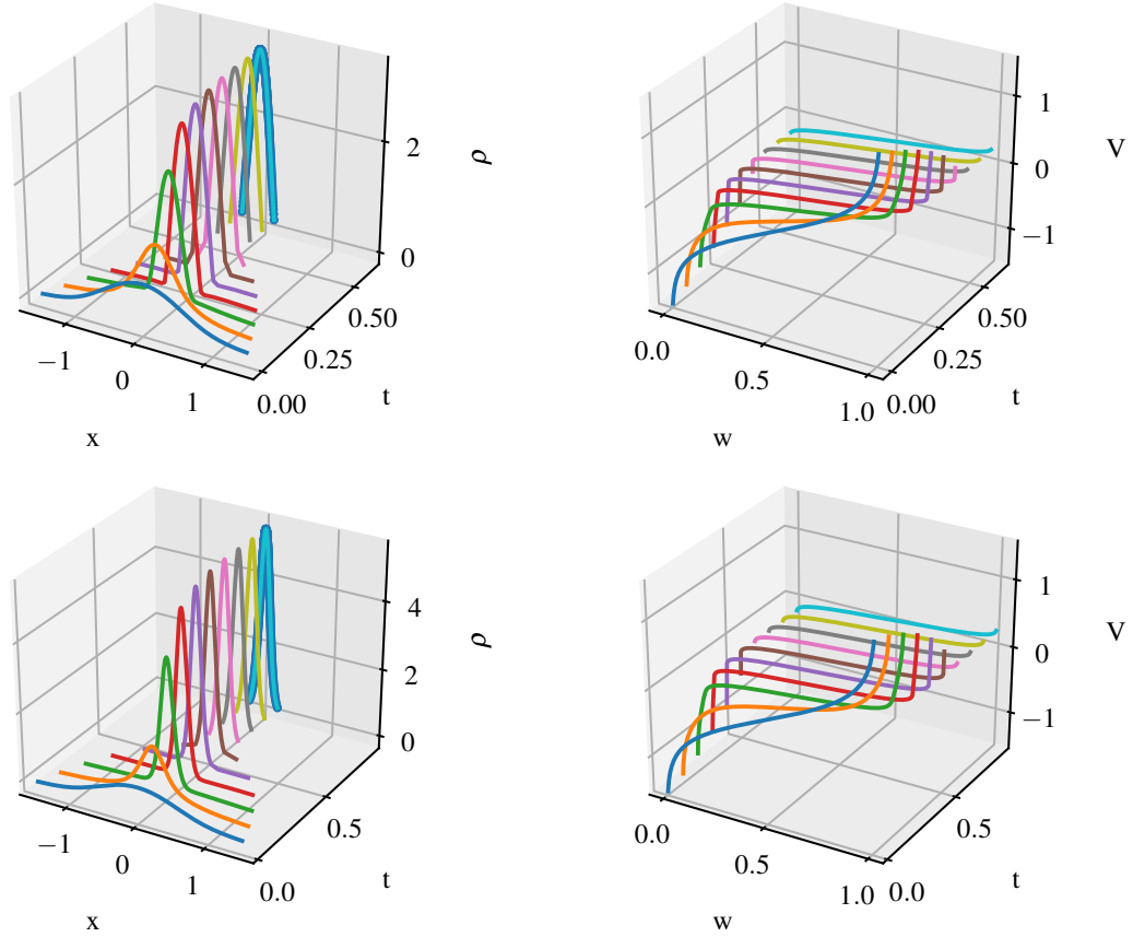
FIGURE 3. Numerical results (cell concentration and inverse cumulative function) for the nonlinear diffusion model (4.4), initial condition (4.3), \chi = 2.5\pi and \gamma = 2 (top row), \gamma = 1.5 (bottom row). For both chosen values of m the numerical solution converges to a steady state. We have used M = 500 points.
