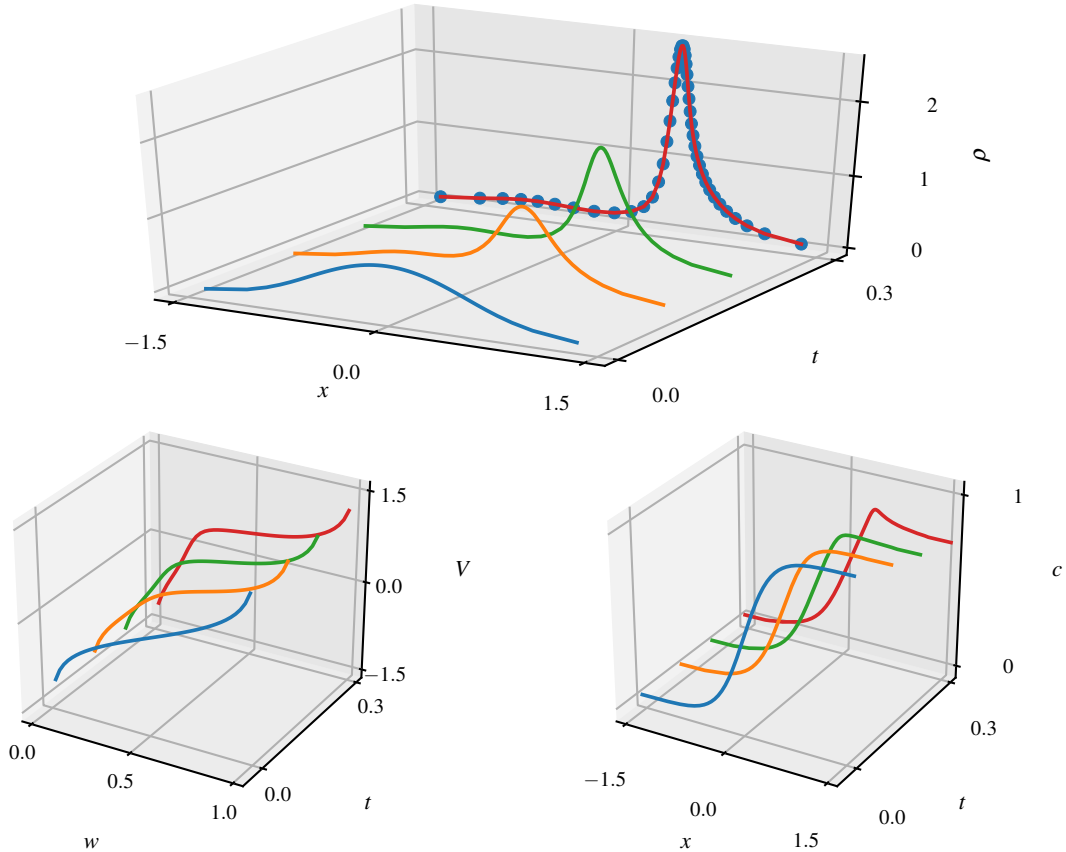
FIGURE 5. Numerical results (cell concentration, inverse cumulative function, and chemo-attractant density in space and time) for the parabolic-parabolic KS model (4.8) in the “peak movement” experiment. The movement and aggregation is accurately resolved using M = 45 grid points.
